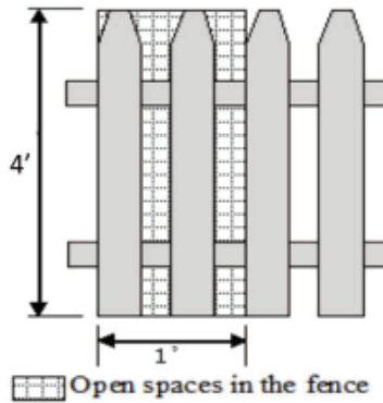
Figure 1, Open Fence Example: For a 4' tall open fence, the open spaces in the fence shall include at least 30% or 1.2 sq. feet per one linear foot in length.
